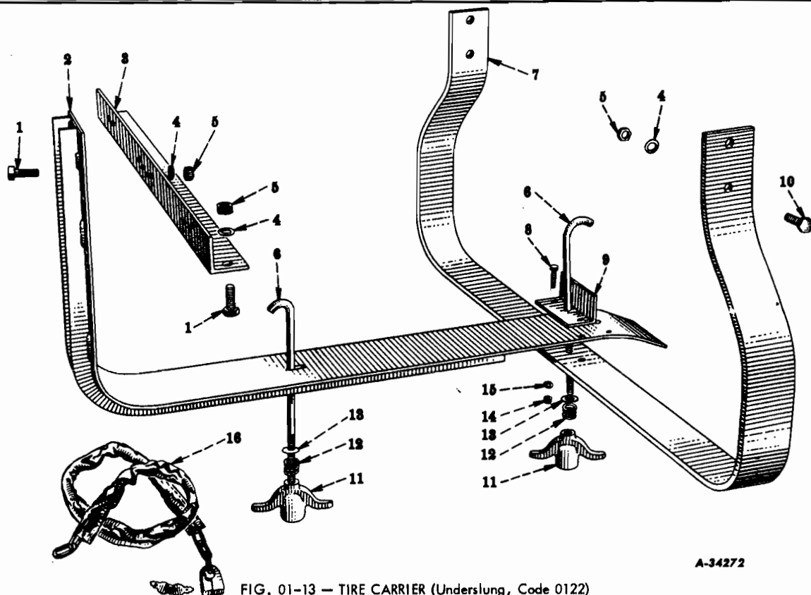
FIG. 01-13 — TIRE CARRIER (Underslung, Code 0122) (R-160 Series)
