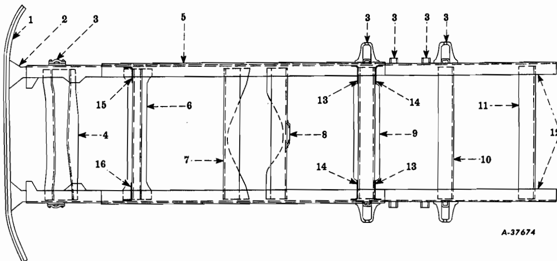
FIG. 01-4 — FRAME ASSEMBLY (R-163)
