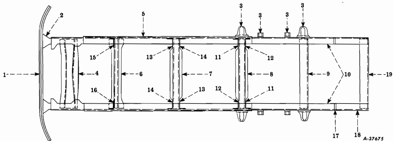
FIG. 01-5 — FRAME ASSEMBLY (RC-160 Series)
