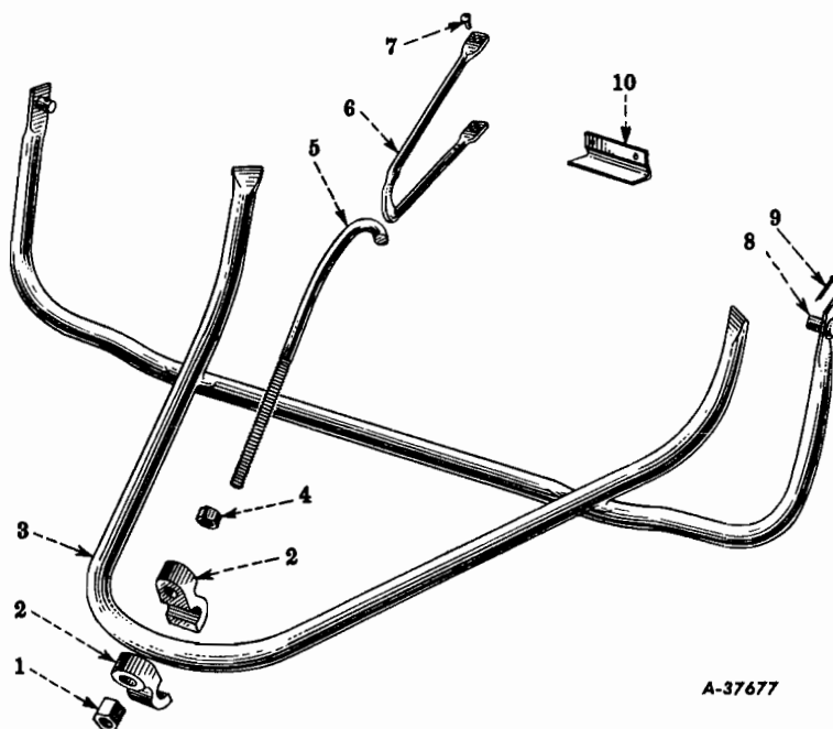
FIG. 01-8 — TIRE CARRIER (Underslung, Code 0121) (Tubular Type) (R-110, R-120 Series) (R-130 Series - With 115, 122" W.B.)
