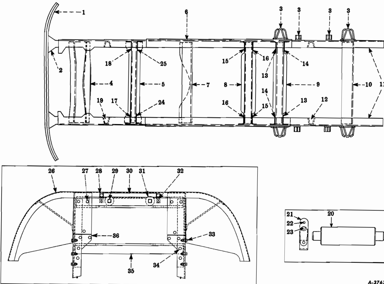
FIG. 01-6 — FRAME ASSEMBLY (R-140-4x4, R-160-4x4 Series)
