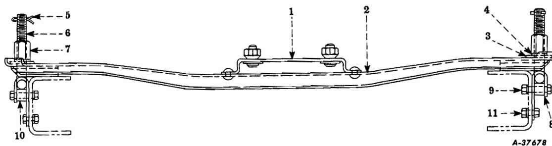
FIG. 01-11 — TIRE CARRIER (Underslung, Code 0121) (Bar Type) (R-130 Series - With 134" W.B.)
