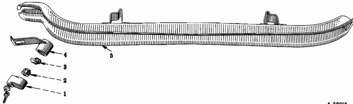
FIG. 01-12 — TIRE CARRIER LOCK (Code 0124) (For Underslung Bar Type Carriers)
