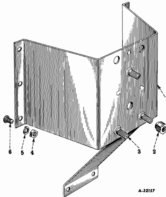
FIG. 01-14 — SPARE TIRE CARRIER (Side Mounted, Code 0130) (R-100, R-110, R-120 Series)
