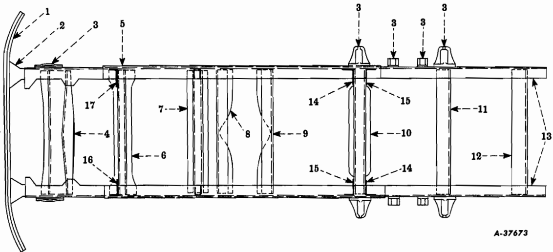
FIG. 01-3 — FRAME ASSEMBLY (R-160, R-164, R-165)
