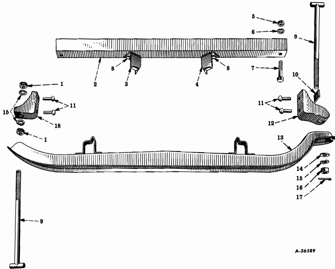
FIG. 01-10 - TIRE CARRIER (Underslung, Code 0121) (Bar Type) (R-140-4x4, R-150, R-160, R-160-4x4, RC-160)
