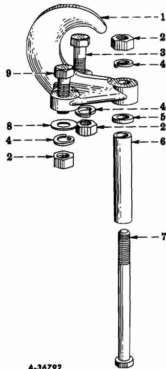
FIG. 01-15 — FRONT TOW HOOKS (Code 0114) (R-140-4x4, R-150, R-160, RC-160 Series)
