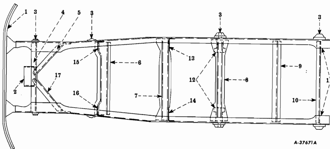
FIG. 01-1 — FRAME ASSEMBLY (R-100, R-110, R-120, R-130 Series)
