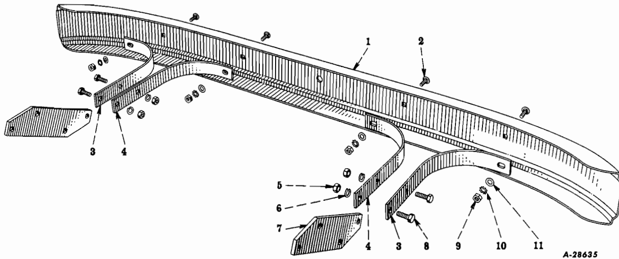
FIG. 01-7 — REAR BUMPER
